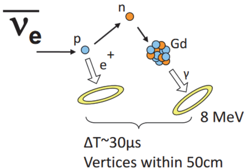
Figure 2: Principle of the delayed coincidence method with gadolinium for antineutrino detection.
